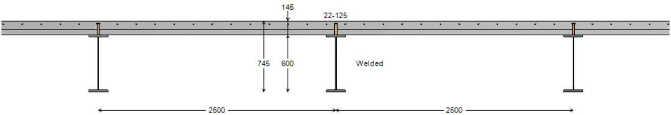
Figure 21 : Transversal view
