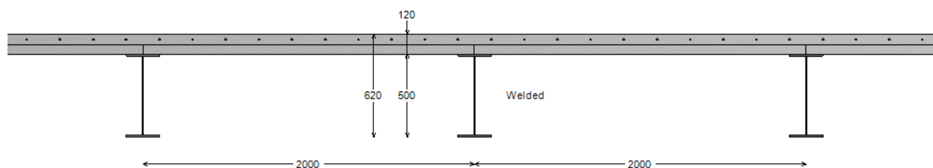
Figure 18 : Transversal view
