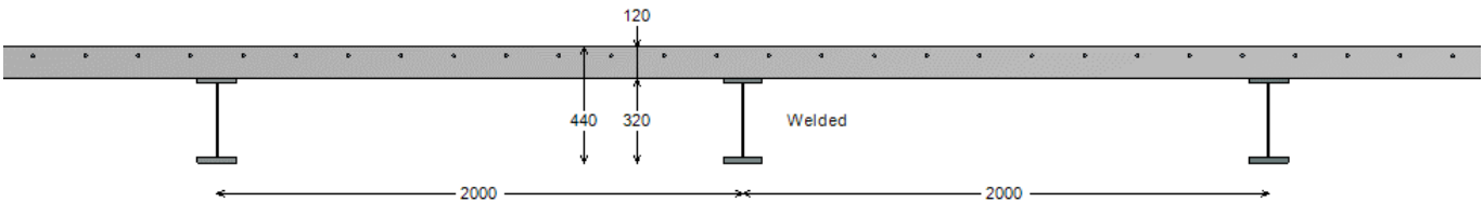
Figure 11 : Transversal view
