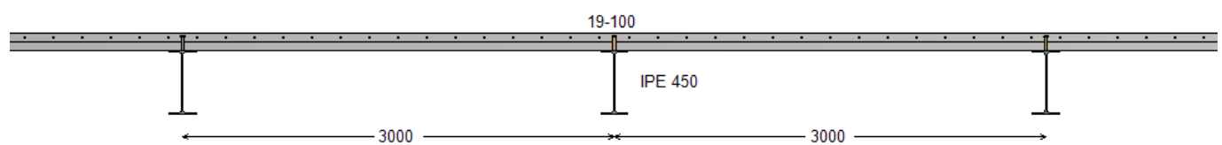
Figure 2 : Transversal view
