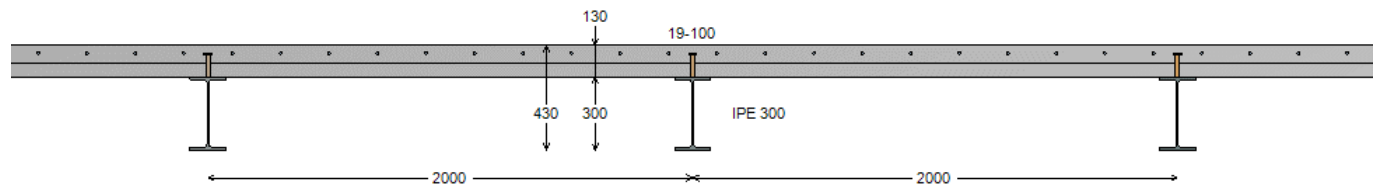
Figure 19 : Transversal view
