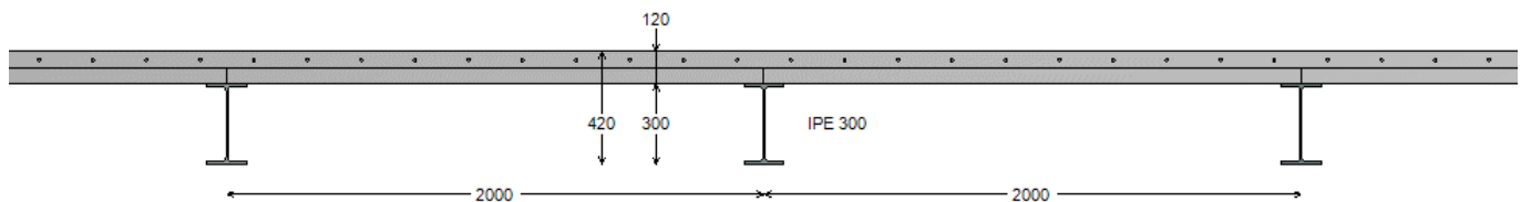
Figure 15 : Transversal view
