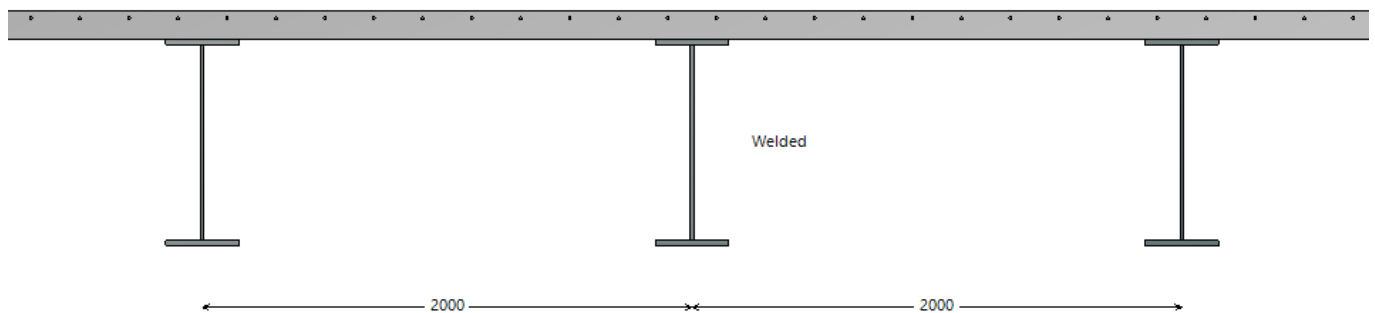
Figure 14 : Transversal view
