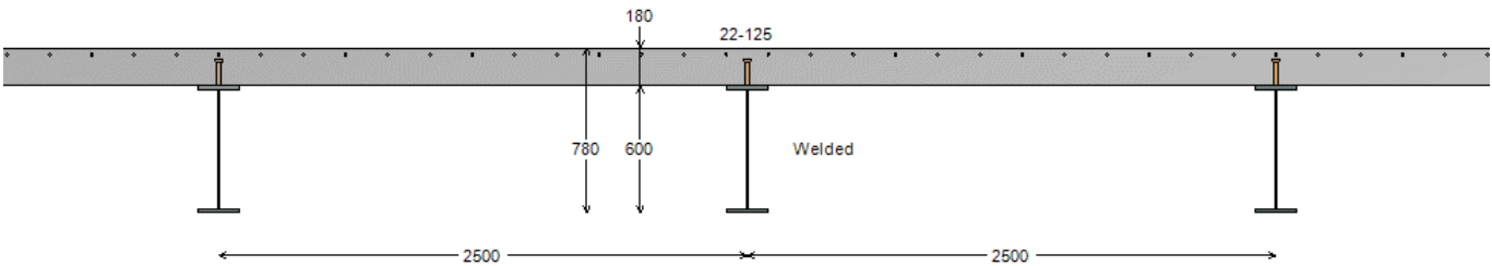
Figure 23 : Transversal view
