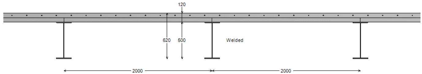
Figure 17 : Transversal view
